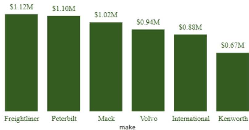
Maintainance Cost by Truck make
